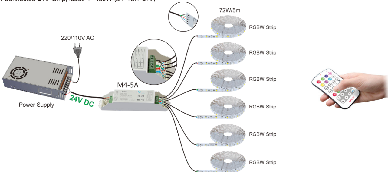
E.g. 2: Connected 24V lamp, loads 1~480W (5A×4CH×24V).
